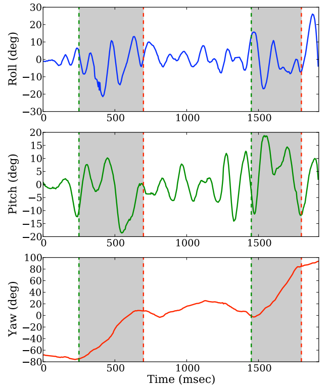
(a) Robot orientation during dynamic turns. Note increases in roll and pitch magnitudes corresponding to sudden changes in yaw.
