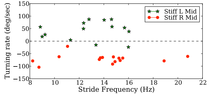
Fig. 9: Turning rate vs. stride frequency
