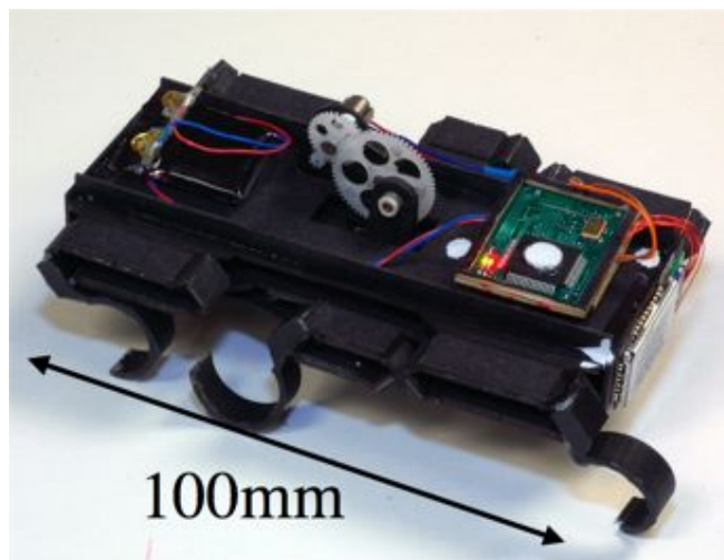
Fig. 1: The DynaRoACH robot.
